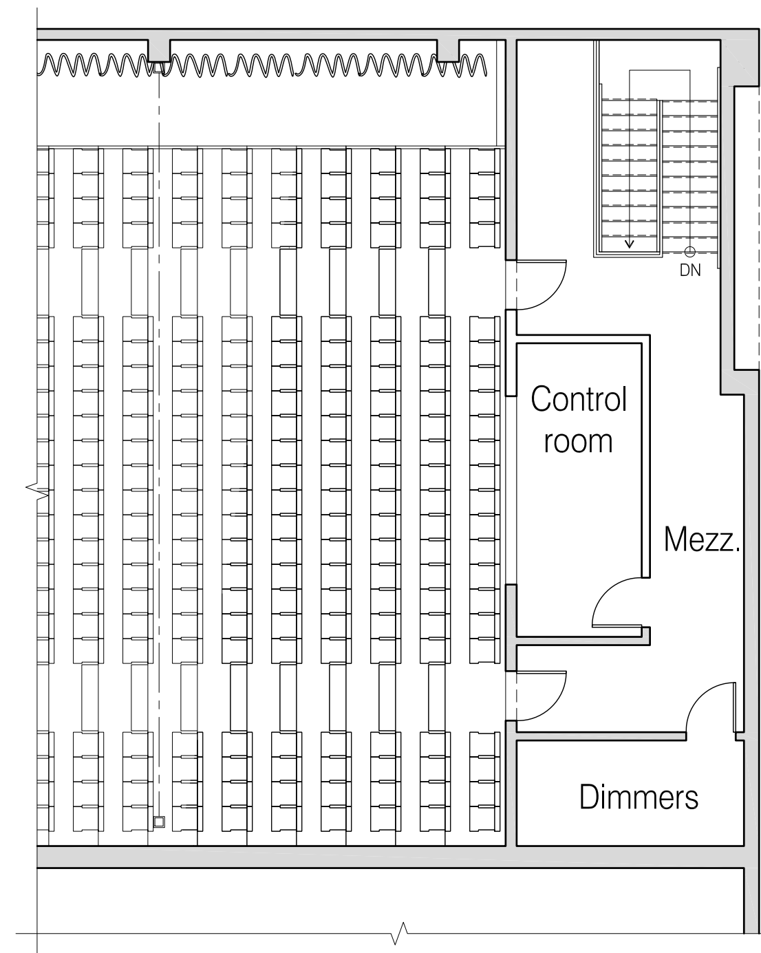
C1 Public Assembly Plan - Mezzanine Lvl. 1/8" = 1'-0"
